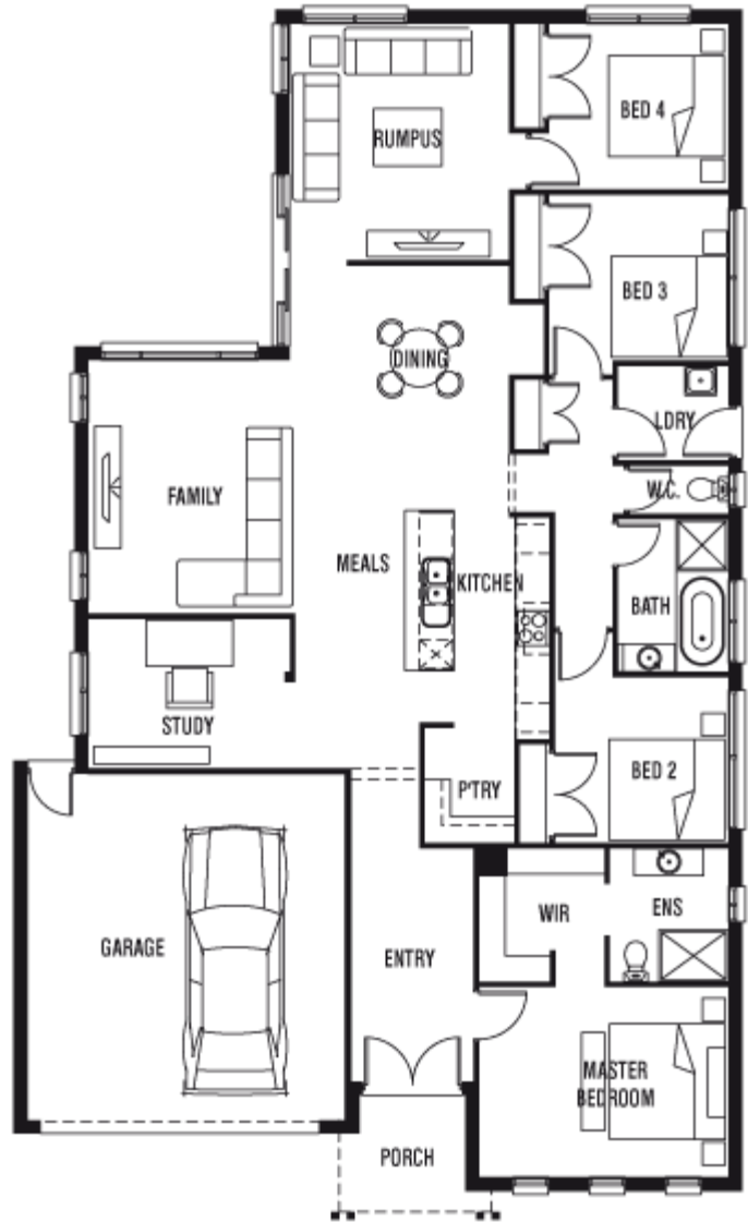
House width 12.60m x House length 21.00m
